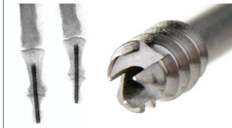
SCRU™2® True headless screw
